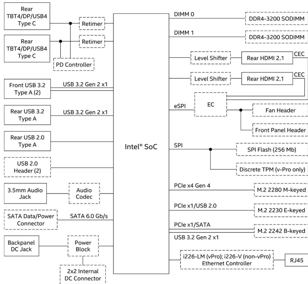
Figure 6. Block Diagram
